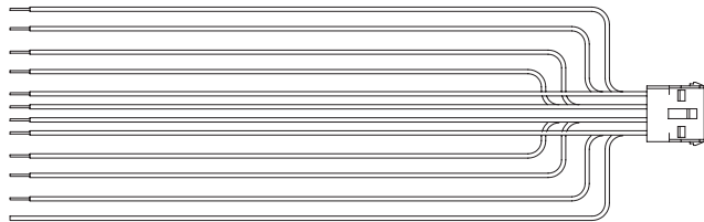
12-PIN POWER/A-B SPEAKER MATING PIGTAIL
